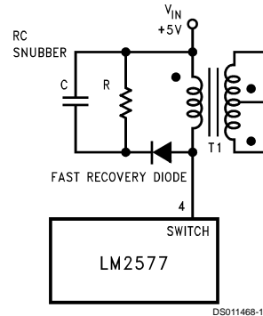
FIGURE 21. Snubber Circuit
