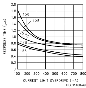
Current Limit Response Time vs Overdrive
