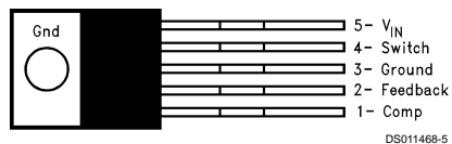
Bent, Staggered Leads 5-Lead TO-220 (T)
