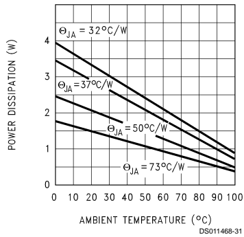
Maximum Power Dissipation (TO-263) (Note 9)
