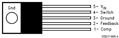
Straight Leads 5-Lead TO-220 (T)
