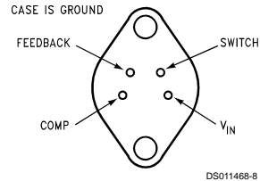
4-Lead TO-3 (K)
