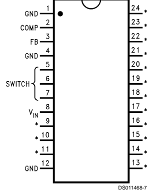
24-Lead Surface Mount (M)
