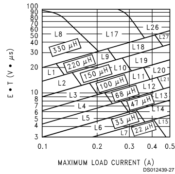
FIGURE 7. LM2594/LM2594HV-ADJ
