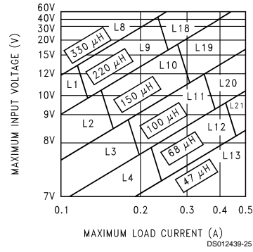
FIGURE 5. LM2594/LM2594HV-5.0
