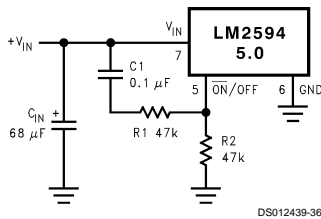
FIGURE 21. Delayed Startup
