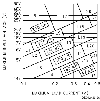
FIGURE 6. LM2594/LM2594HV-12
