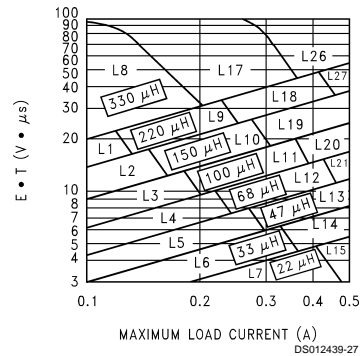
FIGURE 7. LM2594/LM2594HV-ADJ
