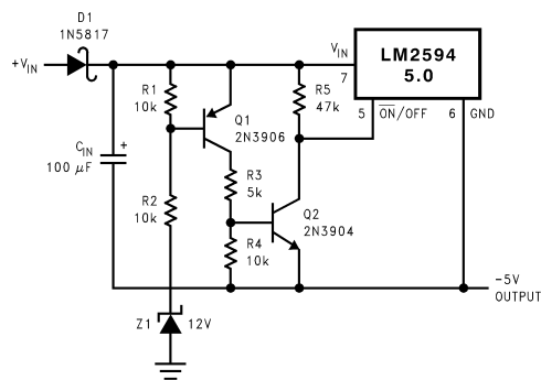
FIGURE 23. Undervoltage Lockout for Inverting Regulator
