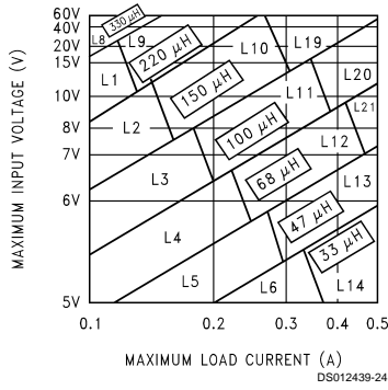
FIGURE 4. LM2594/LM2594HV-3.3
