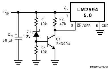
FIGURE 22. Undervoltage Lockout for Buck Regulator
