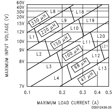
FIGURE 5. LM2594/LM2594HV-5.0
