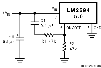
FIGURE 21. Delayed Startup
