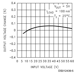
Line Regulation
