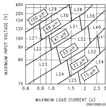
FIGURE 5. LM2596-5.0
