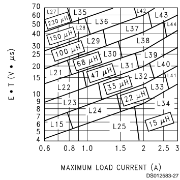
FIGURE 7. LM2596-ADJ
