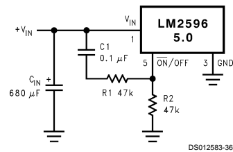
FIGURE 21. Delayed Startup
