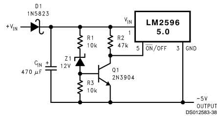
FIGURE 23. Undervoltage Lockout for Inverting Regulator
