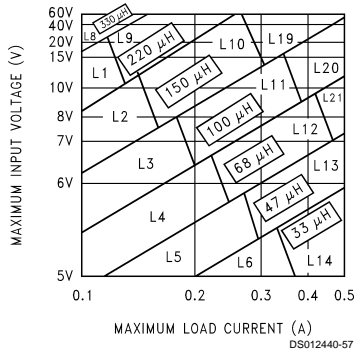
FIGURE 3. LM2597/LM2597HV-3.3
