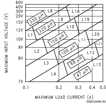
FIGURE 4. LM2597/LM2597HV-5.0
