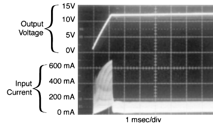
FIGURE 26. Output Voltage, Input Current, at Start-Up, WITHOUT Soft-start
