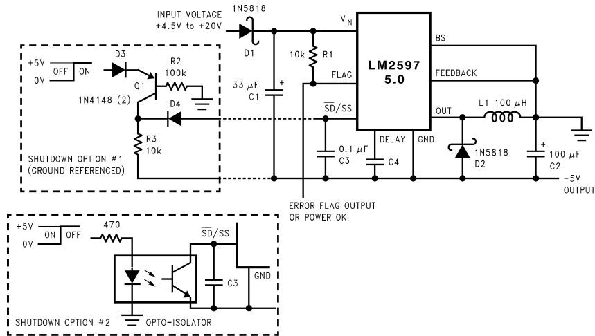
FIGURE 28. Inverting -5V Regulator With Shutdown and Soft-start
