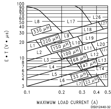
FIGURE 6. LM2597/LM2597HV-ADJ
