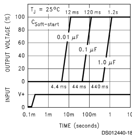
Soft-start Response
