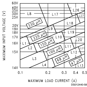
FIGURE 5. LM2597/LM2597HV-12
