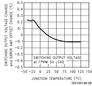
Normalized Switching Output Voltage vs Junction Temperature
