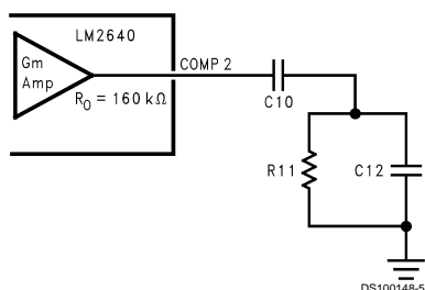
FIGURE 4. Typical Compensation Network
