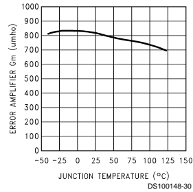
Error Amplifier Gm vs Junction Temperature
