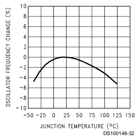
Normalized Oscillator Frequency vs. Junction Temperature
