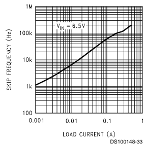
CH1 Skip Frequency vs Load Current
