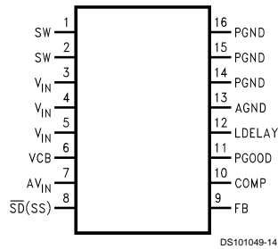
16-Lead TSSOP (MTC)
