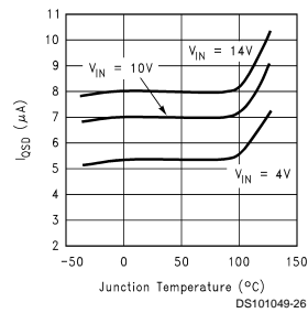
I_{QSD} vs Junction Temperature
