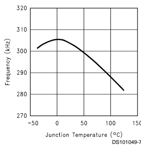
Frequency vs Junction Temperature
