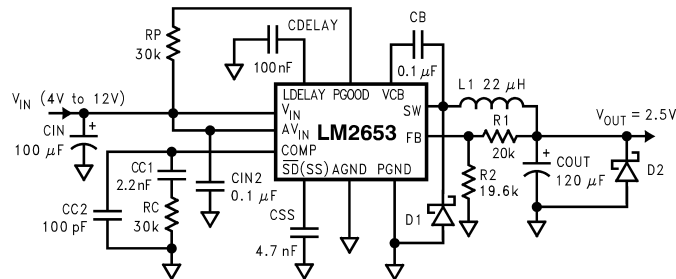
Schematic for the Typical Board Layout
