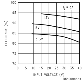
Efficiency vs Input Voltage
