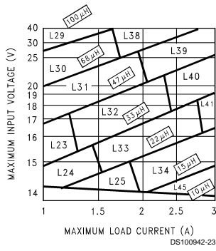
FIGURE 5. LM2670-12
