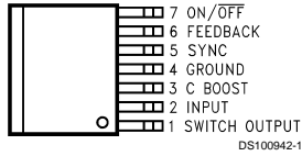
TO-263 Package Top View
