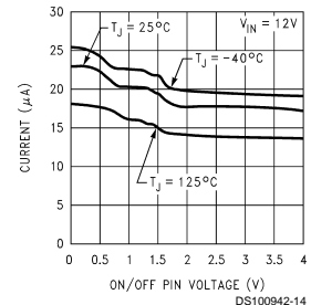
ON/OFF Pin Current (Sourcing)
