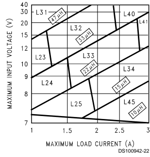
FIGURE 4. LM2670-5.0
