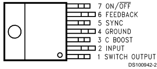
TO-220 Package Top View
