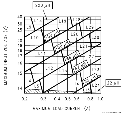
FIGURE 6. LM2675-12
