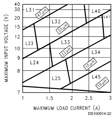
FIGURE 4. LM2676-5.0
