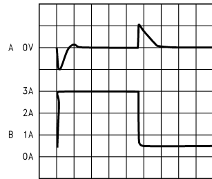
100 \mu sec/Div DS100914-19
