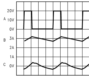
1 \mu sec/Div DS100914-17
