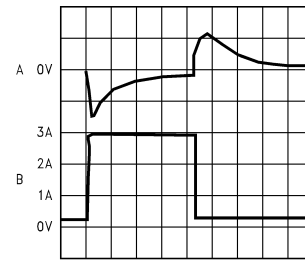
200 \mu sec/Div DS100914-20
