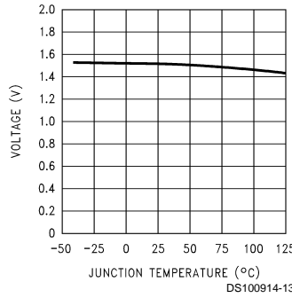
ON/OFF Threshold Voltage
