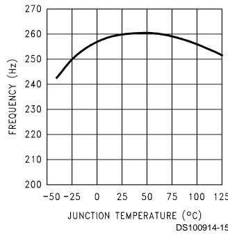
Switching Frequency
