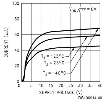
Standby Quiescent Current
