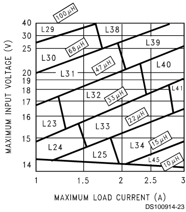
FIGURE 5. LM2676-12
