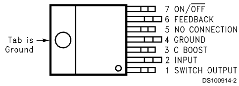
TO-220 Package Top View
