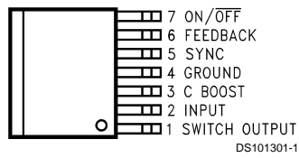
TO-263 Package Top View
