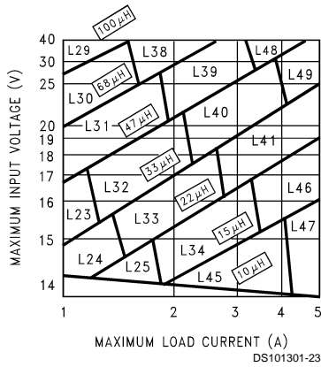
FIGURE 5. LM2677-12
