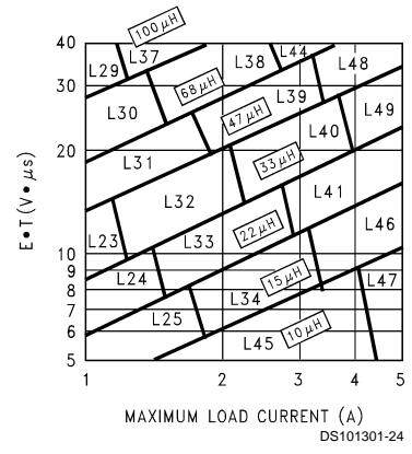
FIGURE 6. LM2677-ADJ
