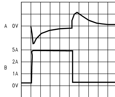
200 \mu sec/Div DS101301-20
