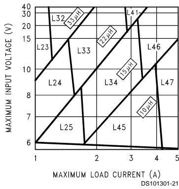
FIGURE 3. LM2677-3.3
