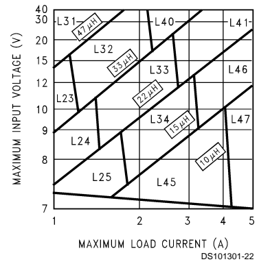
FIGURE 4. LM2677-5.0
