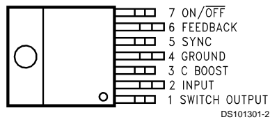
TO-220 Package Top View
