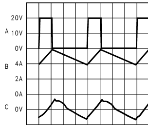
1 \mu sec/Div DS100886-17
