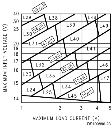
FIGURE 5. LM2678-12
