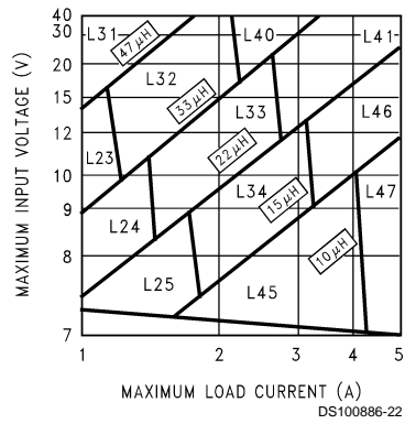
FIGURE 4. LM2678-5.0
