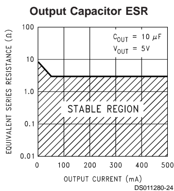
FIGURE 1. ESR Limits
