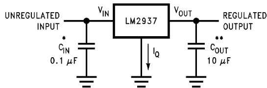
Typical Application
