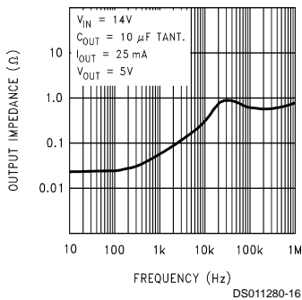
Output Impedance
