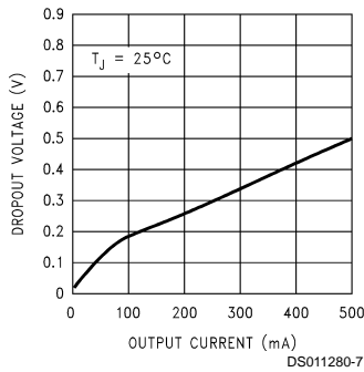
Dropout Voltage vs Output Current
