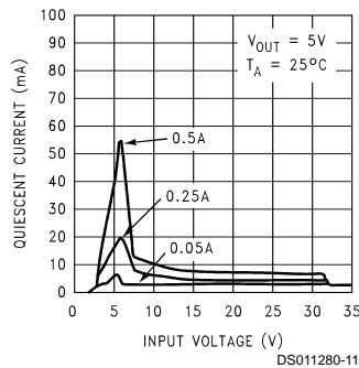
Quiescent Current vs Input Voltage
