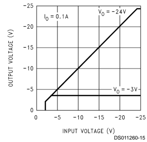
Output Voltage
