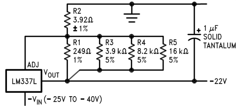
Regulator with Trimmable Output Voltage
