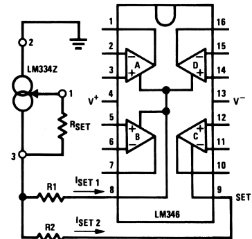
Blasing all 4 Amplifiers with Single Current Source
