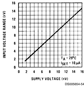
Input Voltage Range vs Supply Voltage
