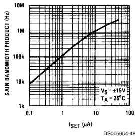
Gain Bandwidth Product vs I_{SET}
