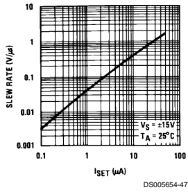
Slew Rate vs I_{SET}
