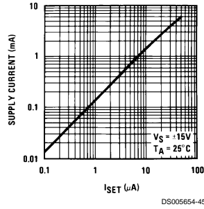
Supply Current vs I_{SET}
