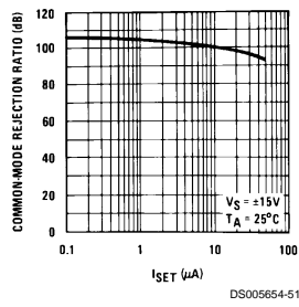
Common-Mode Rejection Ratio vs I_{SET}
