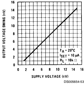
Open Voltage Swing vs Supply Voltage
