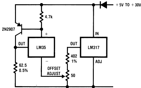
FIGURE 9. 4-To-20 mA Current Source ( 0^{\circ}\text{C} to +100^{\circ}\text{C} )
