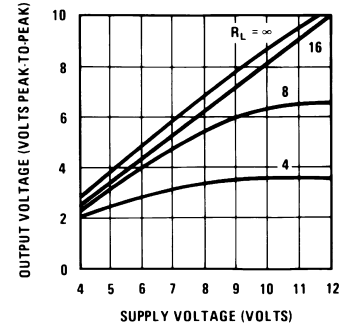
Peak-to-Peak Output Voltage Swing vs Supply Voltage
