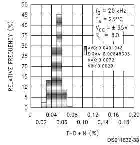
THD+N Distribution
