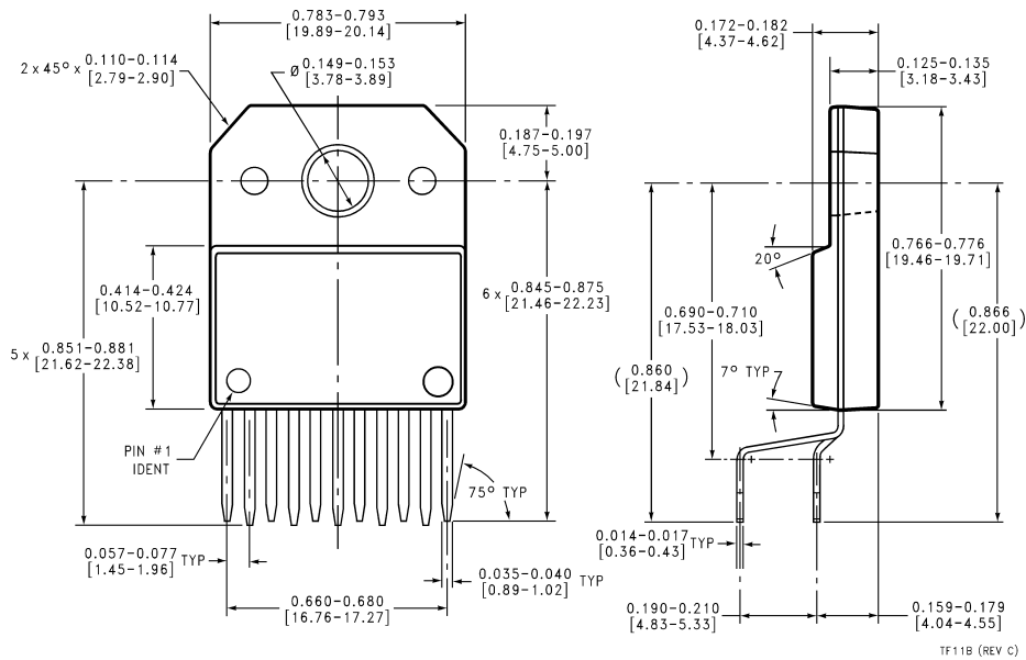
Order Number LM3886TF NS Package Number TF11B
