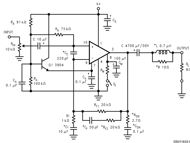
FIGURE 2. Typical Single Supply Audio Amplifier Application Circuit
