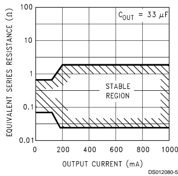
FIGURE 1. ESR Limits
