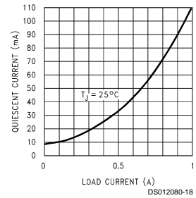
Quiescent Current vs Load
