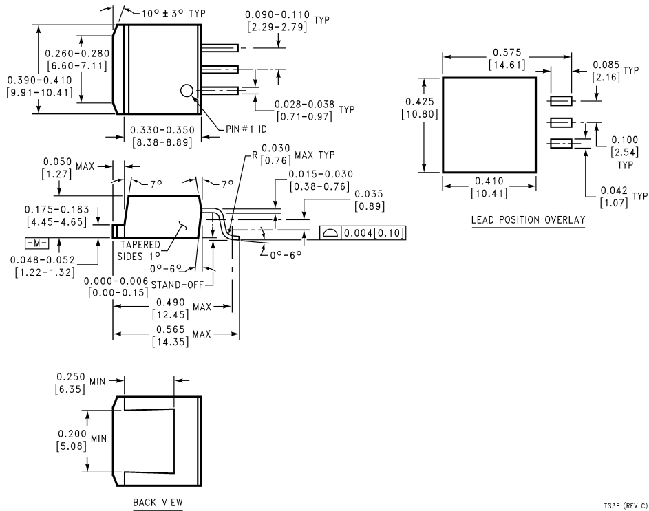
BACK VIEW
