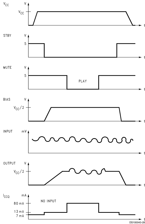
FIGURE 4. Turn-On/Off Sequence
