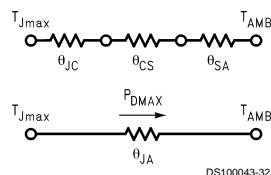
FIGURE 8. Thermal Model
