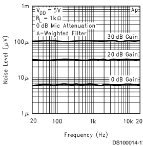
Mic Amplifier Noise Floor
