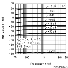
Mic Amplifier Attenuation vs Frequency
