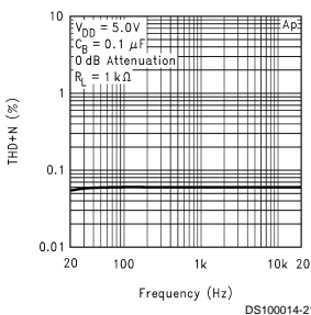
Loop-out THD+N vs Frequency
