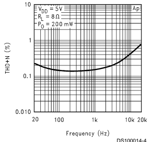
THD+N vs Frequency, 8Ω
