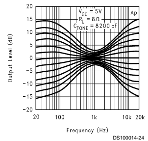
Bass and Treble Response vs Frequency
