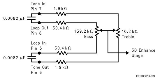
FIGURE 6. Tone Control Diagram
