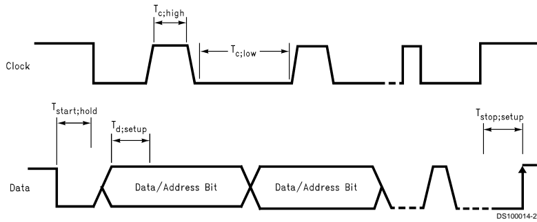
FIGURE 4. I 2 C Timing Diagram
