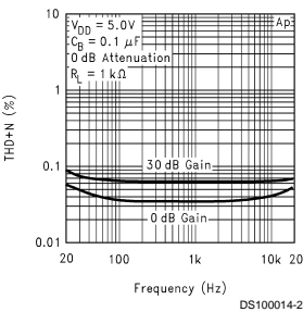
Mic Amplifier THD+N vs Frequency
