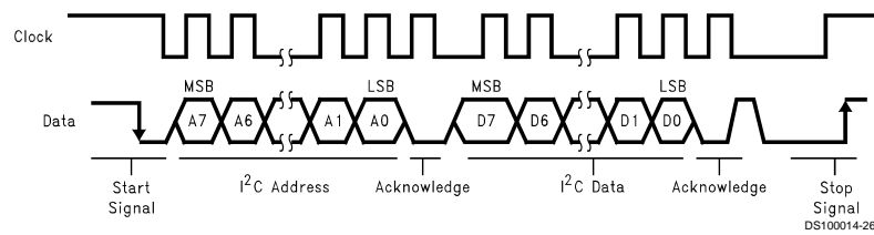
FIGURE 3. I 2 C Bus Format
