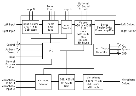
FIGURE 1. LM4832 Block Diagram
