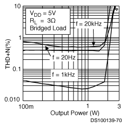
LM4835MTE THD+N vs Output Power
