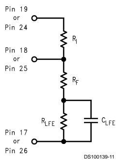
FIGURE 5. Low Frequency Enhancement
