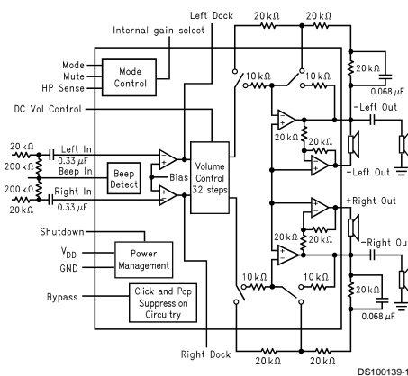
FIGURE 1. LM4835 Block Diagram
