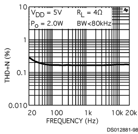
LM4863MTE THD+N vs Frequency
