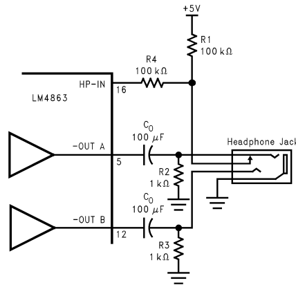
FIGURE 2. Headphone Circuit
