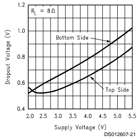
Dropout Voltage vs Supply Voltage
