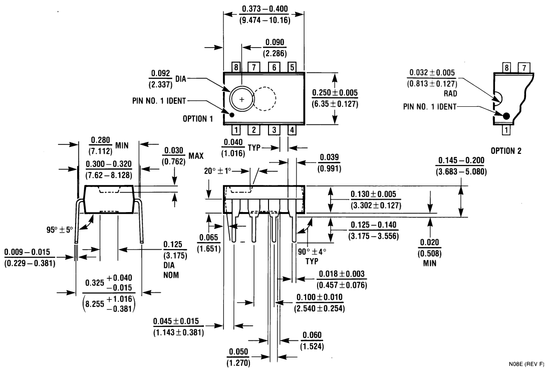
Order Number LM4871N NS Package Number N08E
