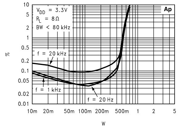
THD+N vs Output Power V DD = 3.3V
