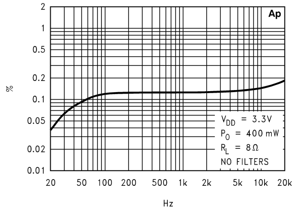
THD+N vs Frequency at 3.3V and 8Ω
