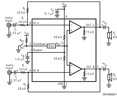
*Refer to the Application Information Section for information concerning proper selection of the input and output coupling capacitors.
