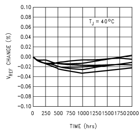
Reference Voltage Drift
