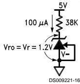
FIGURE 3. 1.2V Reference
