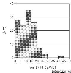
Average V_{OS} Drift Industrial Temperature Range
