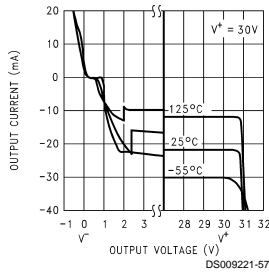
Output Sink Current vs Output Voltage
