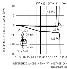
Reference Change vs Common-Mode Voltage
