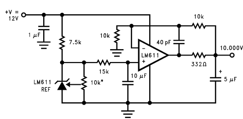
FIGURE 12. Ultra Low Noise 10.000V Reference. Total Output Noise is Typically 14 \mu\text{V}_{\text{RMS}} . Adjust the 10k pot for 10.000V.
