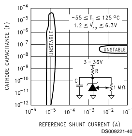
Reference AC Stability Range
