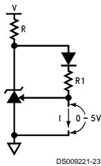
FIGURE 10. Proportional-to-Absolute-Temperature Current Source
