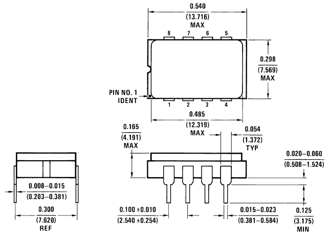
8-Pin Ceramic Sidebrazed Dual-In-Line Package Order Number LM6142AMJ-QML NS Package Number D08C
