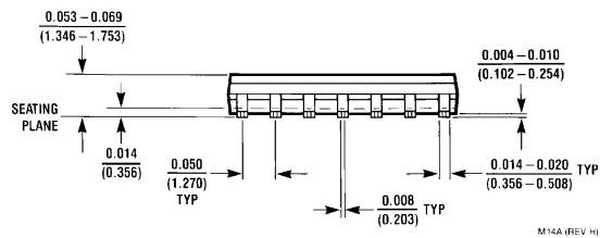
14-Lead (0.150") Molded Small Outline Package, JEDEC Order Number LM6154ACM or LM6154BCM NSC Package Number M14A
