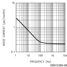
Noise Current vs. Frequency
