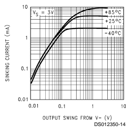
Output Voltage vs. Sink Current
