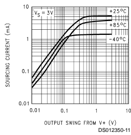
Output Voltage vs. Source Current
