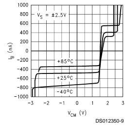
Bias Current vs. V_{CM}
