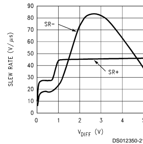
FIGURE 2. Slew Rate vs. V_{diff}
