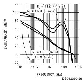
Open Loop Gain/Phase (VS = 24V)
