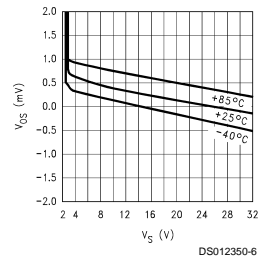
Offset Voltage vs. Supply Voltage
