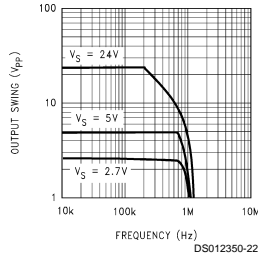
Voltage Swing vs. Frequency (CL = 100 pF)
