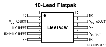
Top View NS Package Number W10A
