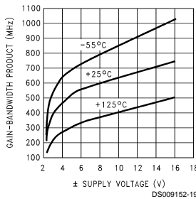
Gain-Bandwidth Product
