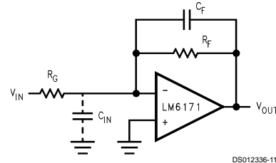
FIGURE 1. Compensating for Input Capacitance
