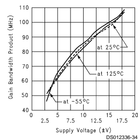
Gain Bandwidth Product vs Supply Voltage
