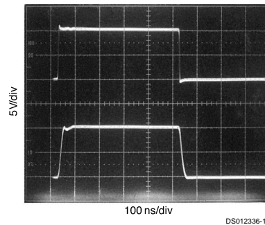
FIGURE 6. The LM6171 Driving a 200 pF Load with a 50 \Omega Isolation Resistor
