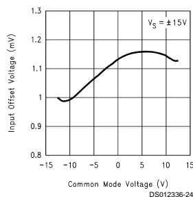
Input Offset Voltage vs Common Mode Voltage
