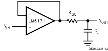
FIGURE 5. Isolation Resistor Used to Drive Capacitive Load
