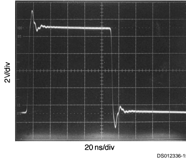
FIGURE 4. Improperly Terminated Signal
