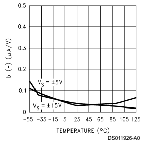
Ib (+) PSR vs Temperature
