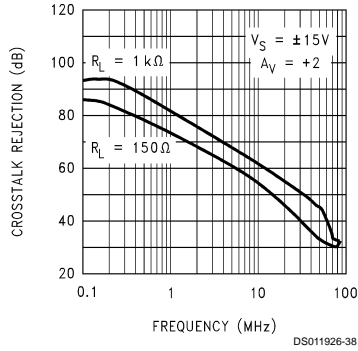
FIGURE 12. Crosstalk Rejection
