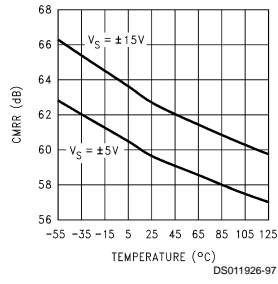
CMRR vs Temperature
