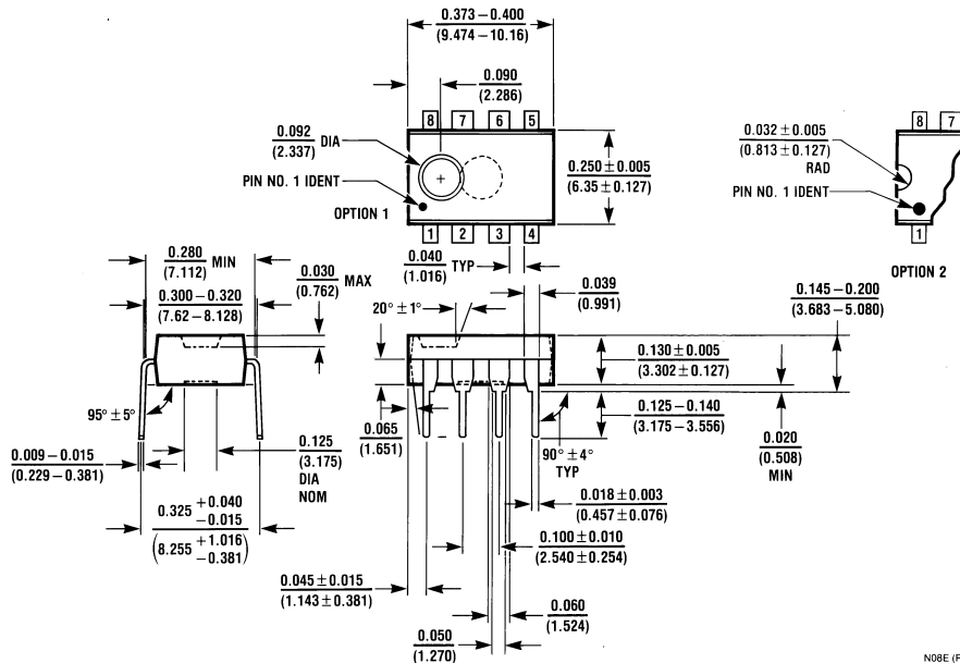
Dual-In-Line Package (N) Order Number LM6182IN, LM6182AIN, or LM6182AMN NS Package Number N08E
