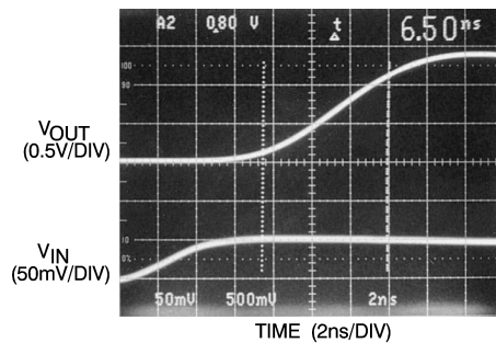
4B. R_f = 500\Omega
