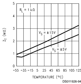
Z_t vs Temperature
