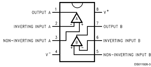
Dual-In-Line Package (N)
