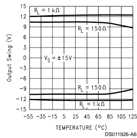
Output Swing vs Temperature
