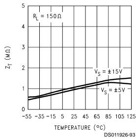
Z_t vs Temperature
