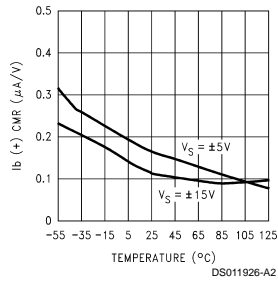
Ib (+) CMR vs Temperature
