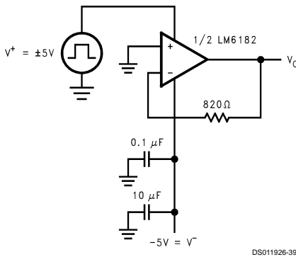
FIGURE 13. Start-Up Test Circuit
