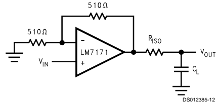
DS012385-12 FIGURE 5. Isolation Resistor Used to Drive Capacitive Load
