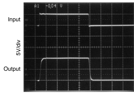
DS012385-13 100 ns/div FIGURE 6. The LM7171 Driving a 150 pF Load with a 50Ω Isolation Resistor
