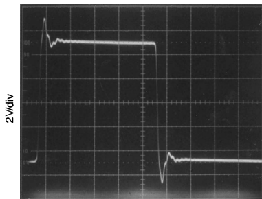
DS012385-18 20 ns/div
