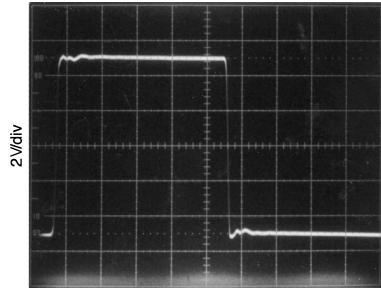
DS012385-17 20 ns/div
