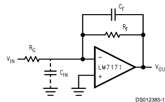
FIGURE 1. Compensating for Input Capacitance
