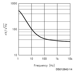
Voltage Noise vs Frequency
