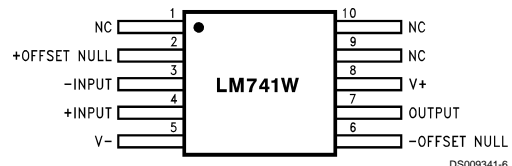
Ceramic Flatpak
