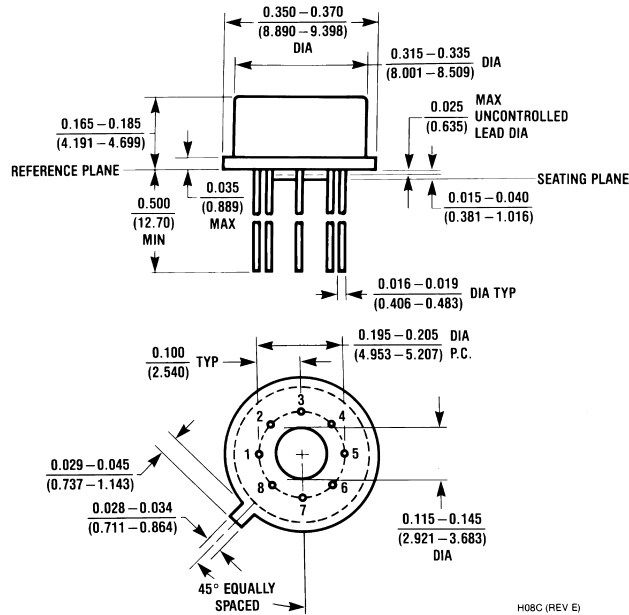
Metal Can Package (H) Order Number LM741H, LM741H/883, LM741AH/883, LM741CH or LM741EH NS Package Number HO8C
