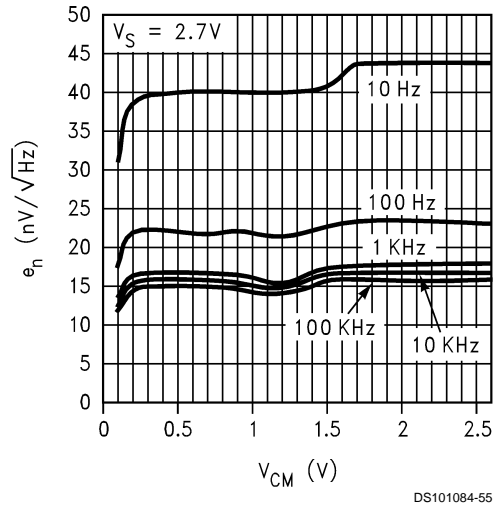
Input Noise Voltage vs. V_{CM}
