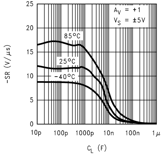
-SR vs. Cap Load
