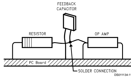
FIGURE 10. Air Wiring
