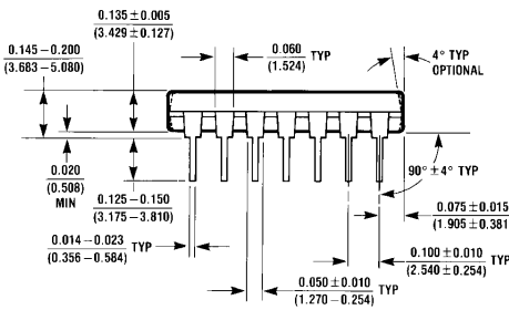
Molded Dual-In-Line Pkg. (N) Order Number LMC6034IN NS Package Number N14A
