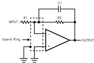
FIGURE 6. Guard Ring Connections Inverting Amplifier
