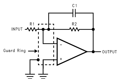
Inverting Amplifier
