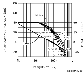
Gain and Phase Responses vs Load Capacitance
