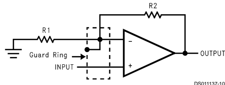
Non-Inverting Amplifier
