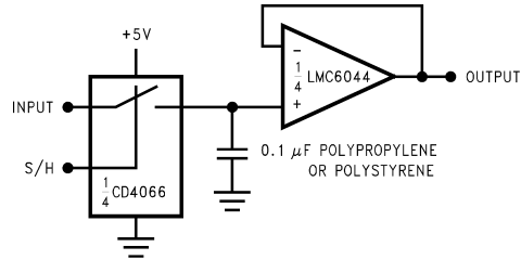
FIGURE 9. Low-Leakage Sample-and-Hold
