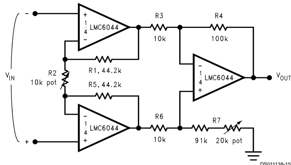
FIGURE 10. Instrumentation Amplifier
