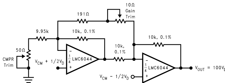
FIGURE 8. Low-Power Two-Op-Amp Instrumentation Amplifier
