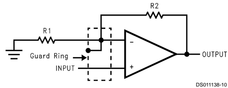
Non-Inverting Amplifier
