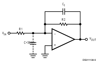
FIGURE 1. Canceling the Effect of Input Capacitance
