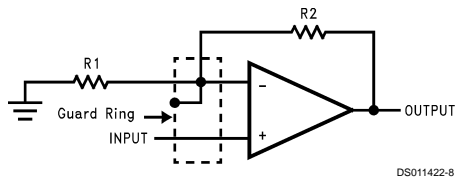
Non-Inverting Amplifier
