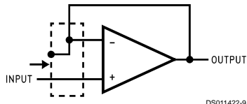
Follower
