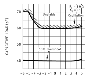
OUTPUT VOLTAGE (V) DS011422-35
