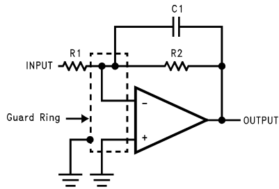
Inverting Amplifier
