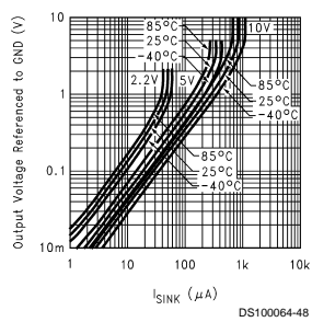
Output Sink Current vs Output Voltage
