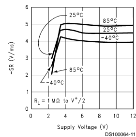
Negative Slew Rate vs Supply Voltage
