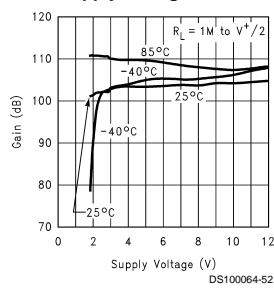
Large Signal Voltage Gain vs Supply Voltage
