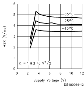
Positive Slew Rate vs Supply Voltage
