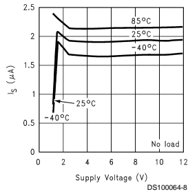
Total Supply Current vs Supply Voltage
