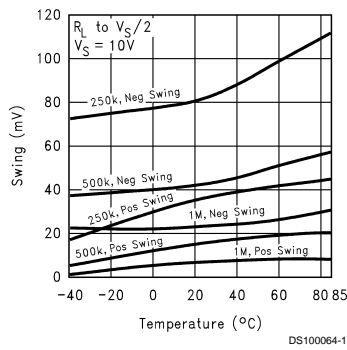
Swing From Rail(s) vs Temperature
