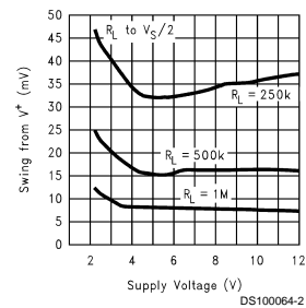
Swing Towards V^+ vs Supply Voltage
