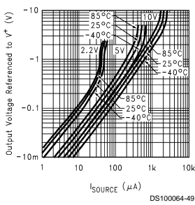
Output Source Current vs Output Voltage
