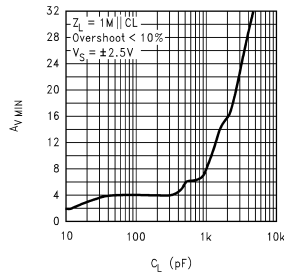
FIGURE 4. Minimum Operating Gain vs Capacitive Load
