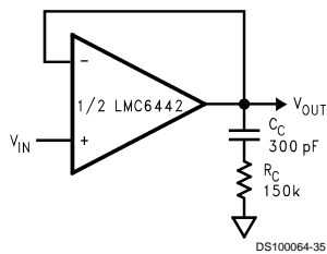
FIGURE 1. A_V = +1 Operation by adding C_C and R_C
