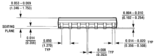
14-Pin Small Outline Package Order Number LMC6464AIM or LMC6464BIM NS Package Number M14A
