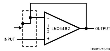
Follower
