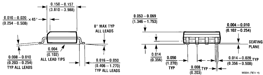
8-Pin Small Outline Package Order Package Number LMC6482AIM or LMC6482IM NS Package Number M08A
