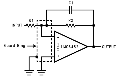
Inverting Amplifier
