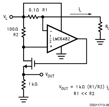
FIGURE 22. Positive Supply Current Sense
