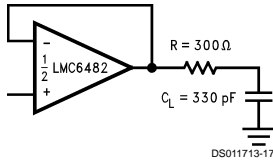
FIGURE 4. Resistive Isolation of a 330 pF Capacitive Load
