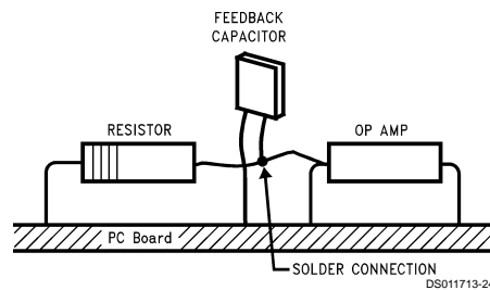
FIGURE 11. Air Wiring
