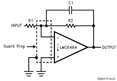
Inverting Amplifier
