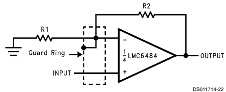
Non-Inverting Amplifier
