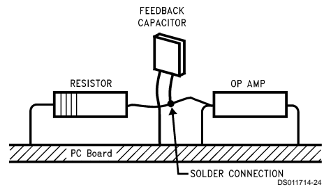
FIGURE 11. Air Wiring
