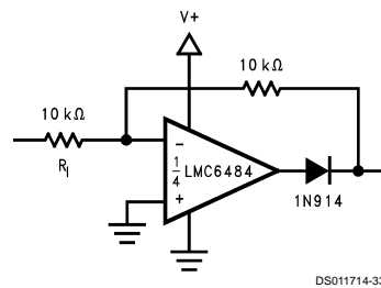
FIGURE 19. Full Wave Rectifier with Input Current Protection ( R_1 )
