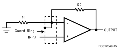
Non-Inverting Amplifier
