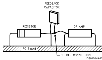
FIGURE 8. Air Wiring
