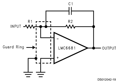
Inverting Amplifier
