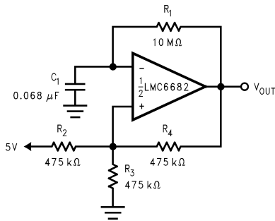
FIGURE 22. 1 Hz Square—Wave Oscillator
