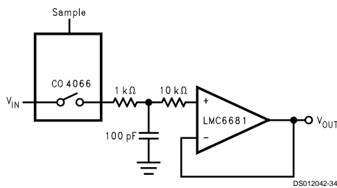
FIGURE 25. Sample-and-Hold Application
