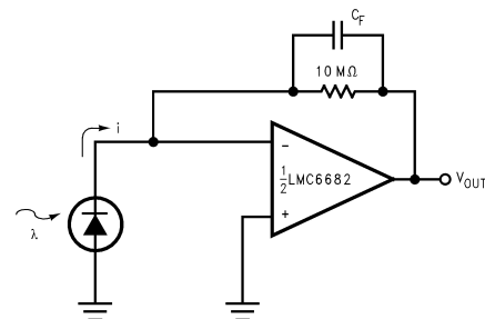
FIGURE 20. Photodiode Amplifier
