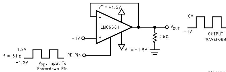
FIGURE 14. Test Circuit for t_{ON} and t_{OFF} Measurements
