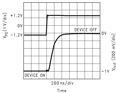
(a) t_{OFF} Measurement
