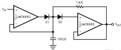
FIGURE 21. Low Voltage Peak Detector
