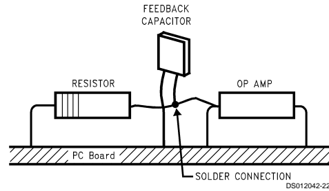
FIGURE 13. Air Wiring
