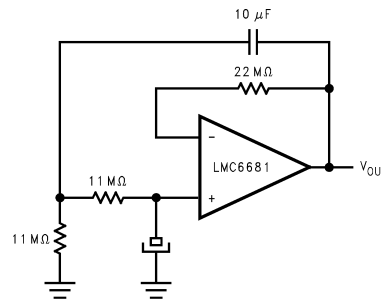
FIGURE 19. LMC6681 Used for Signal Processing
