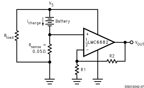
FIGURE 26. Circuit Used to Sense Charging
